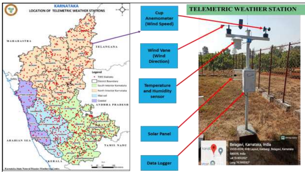
Fig 9: Telemetric Weather Stations network across the State
